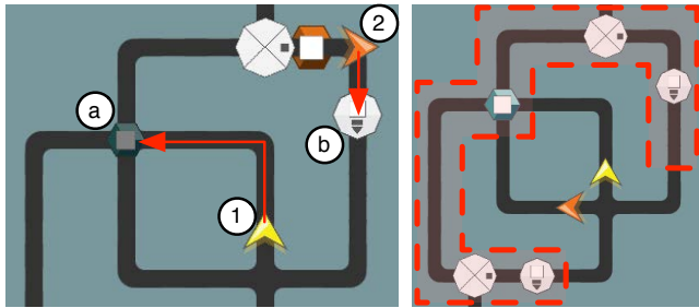
Race Condition: If Arrow 1 arrives to (a) before Arrow 2 arrives to (b), execution will fail. Critical Section: Only one arrow at a time should be allowed in it.
