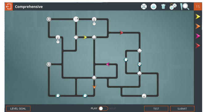
Figure 2: A screen shot of Parallel , in a level with four arrows (four threads) representing the concepts of race condition and of message passing (represented by what we call exchange points).
