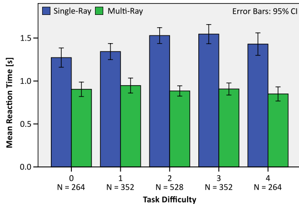
Figure 6: Mean reaction times with 95% confidence intervals over N = 22 \cdot 40 \cdot 2 = 1760 trials in the Single-Ray (blue) and Multi-Ray conditions (green) separated by expected task difficulty.
