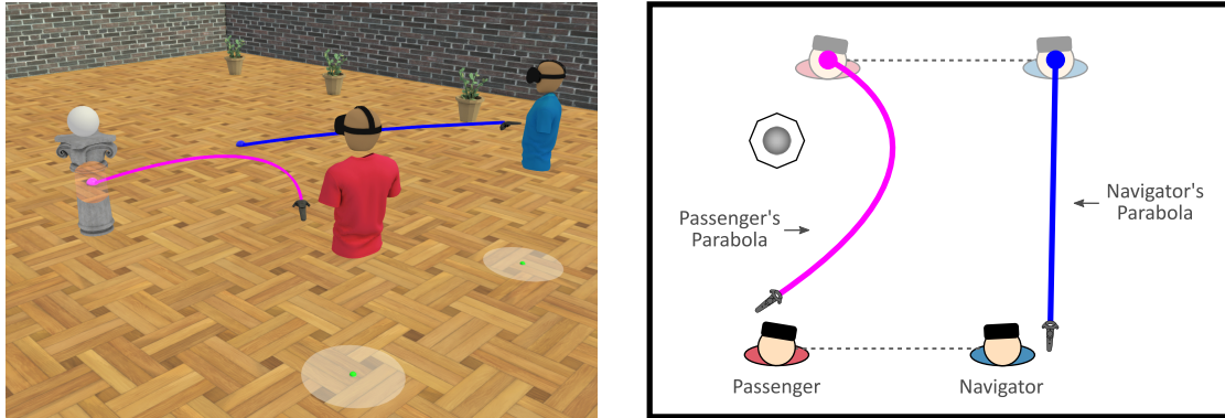
Figure 1: Target specification with Multi-Ray Jumping for two collocated users. While the navigator (blue shirt, right side) specifies a target using the blue parabola, the magenta curve adjusts accordingly to show the offset target location of the passenger (red shirt, left side). The initial direction of the magenta curve is defined by the passenger's controller.
