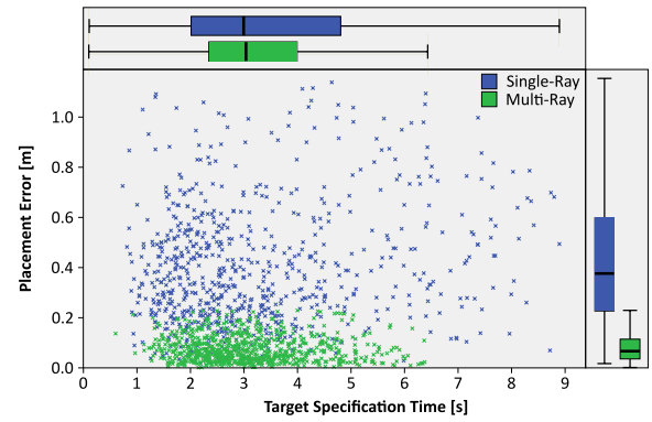
Figure 7: Time-Accuracy scatterplot of all trials of the navigator task without outliers and extreme values ( N = 1760 - 221 = 1539 ). Additional boxplots show the distributions of values in the Single-Ray (blue) and Multi-Ray (green) conditions for both variables.
